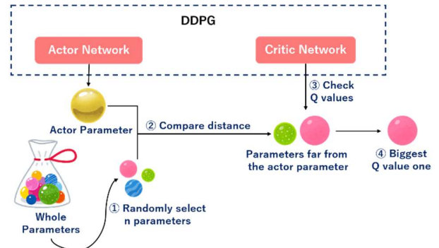
Fig. 12. Flow of selecting the noised action in the stochastic noise policy
