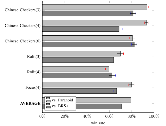
Fig. 9: Performance of MCTS with progressive widening and opponent move abstraction vs. Paranoid and BRS+. 250ms per move.
