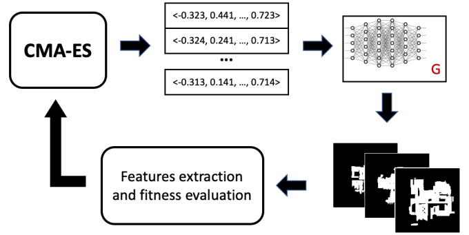
Fig. 3. An overview of our approach for searching the latent space of GAN to generate DOOM levels.
