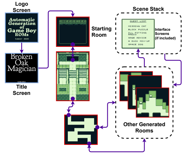
Fig. 4. Diagram of the basic layout of Broken Oak Magician , a generated game. Execution begins with the intro and title screens (top left), from which the player can start a new game or load a saved game. New games start in the scene the generator has designated as the starting room. The scenes are connected via scripts on trigger volumes, creating bidirectional links. Additional interface scenes and modes (menus, combat, etc.) can be accessed using GB Studio’s scene stack, but Broken Oak Magician doesn’t use these more advanced scene-switching features.
