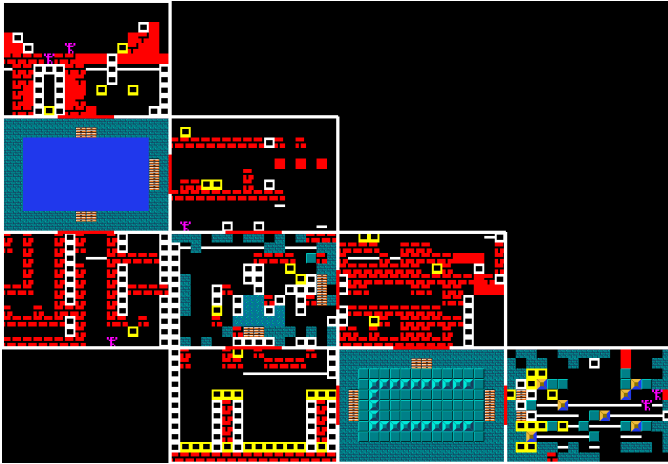
Fig. 5: Example blended Zelda-Lode Runner level.
